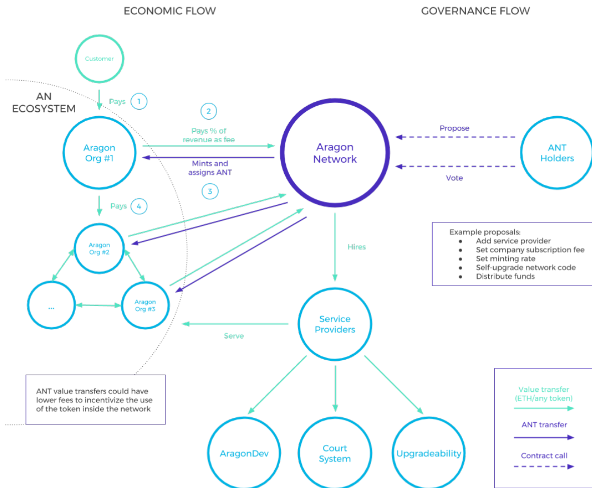
Figure 6: The Aragon Network flow
